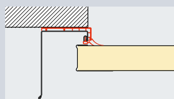
Lintel sealing
