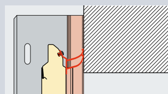
Side sealing
